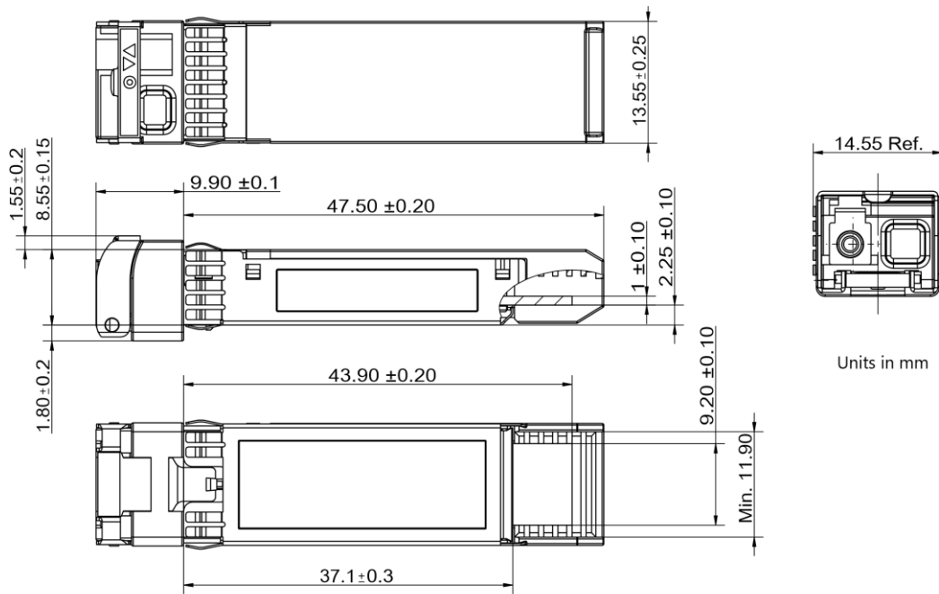
Figure2. Mechanical Outline
